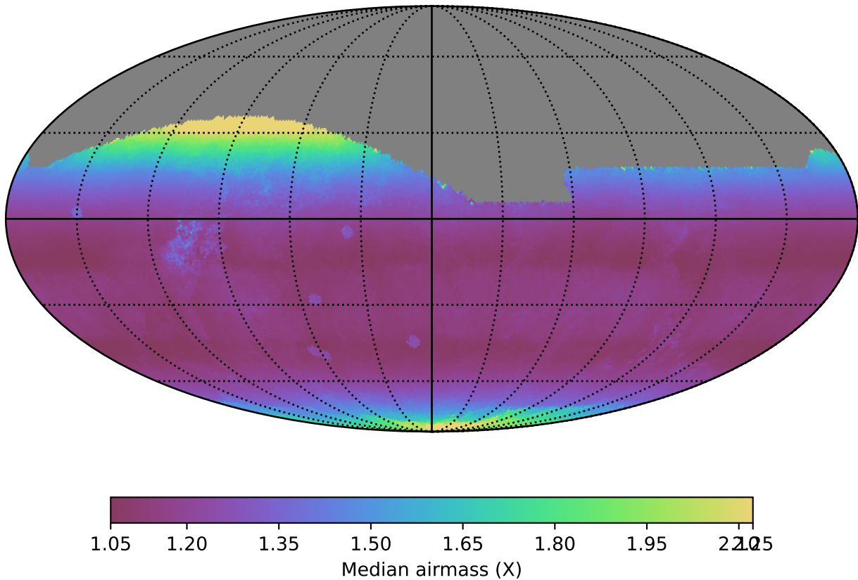
ddf_loaded_fl8_v3.4_10yrs All sky r band: Median airmass
