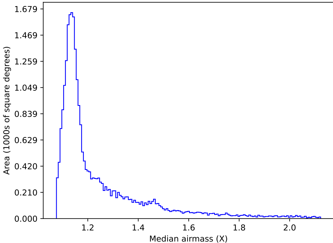
ddf_loaded_fl8_v3.4_10yrs All sky r band: Median airmass
