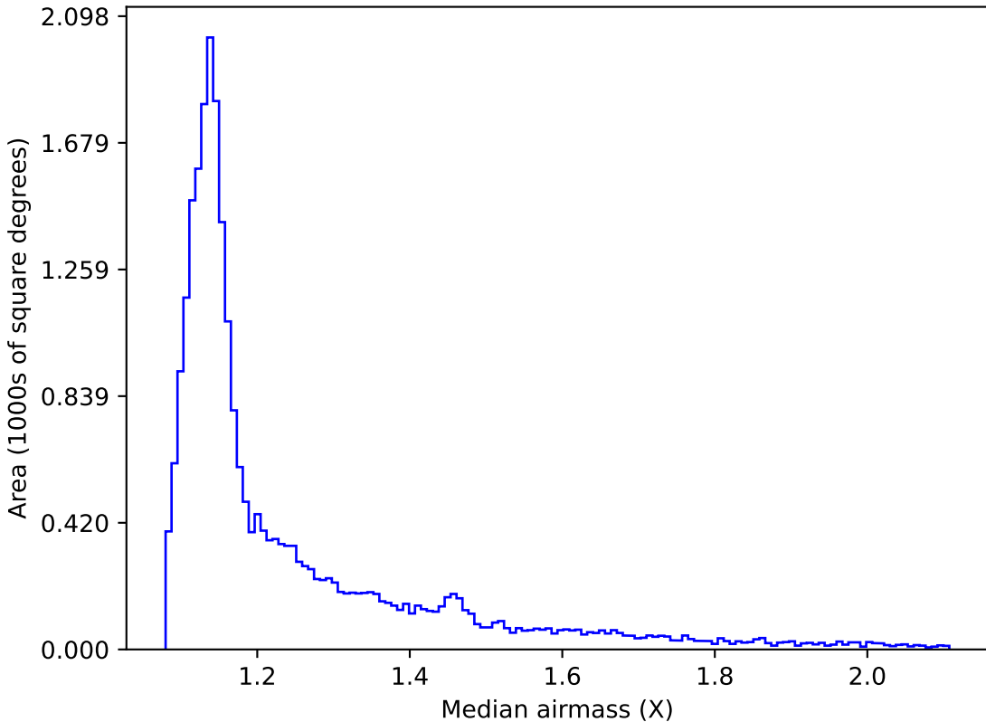
ddf_loaded_fl8_v3.4_10yrs All sky i band: Median airmass
