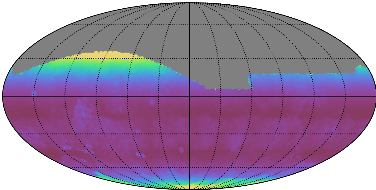
ddf_loaded_fl8_v3.4_10yrs All sky g band: Median airmass
