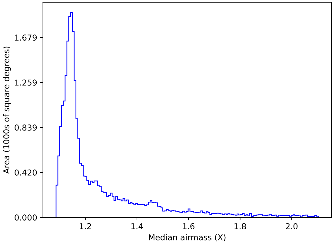
ddf_loaded_fl8_v3.4_10yrs All sky all bands: Median airmass
