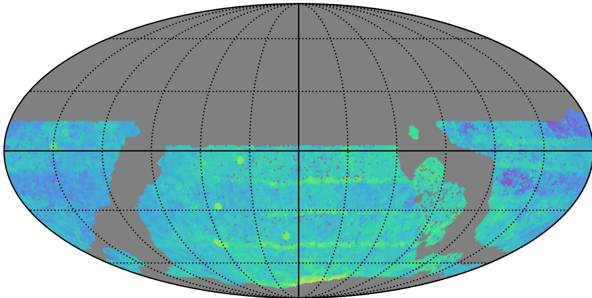
ddf_loaded_fl8_v3.4_10yrs WFD z band: Median Season Length
