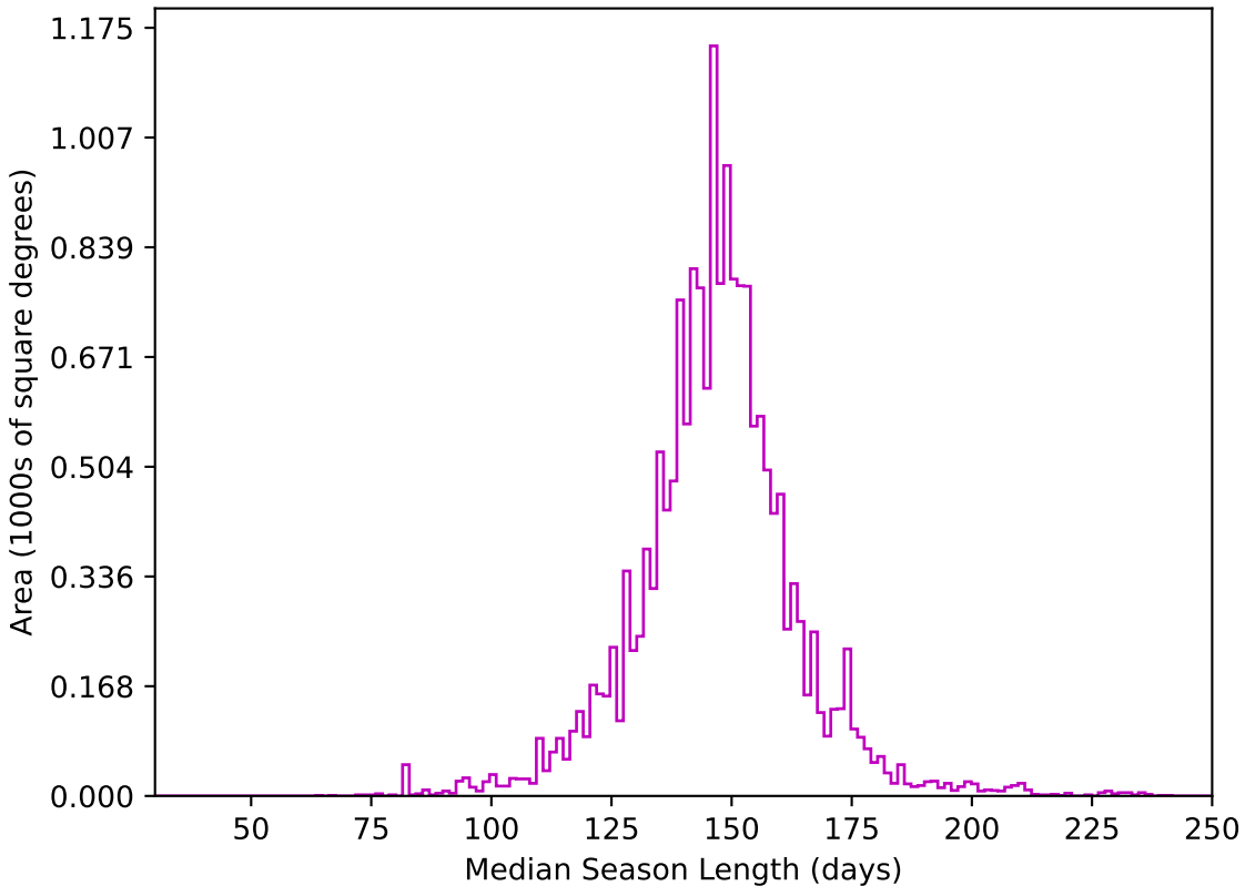
ddf_loaded_fl8_v3.4_10yrs WFD z band: Median Season Length
