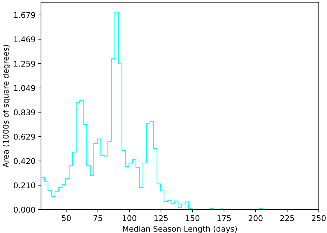
ddf_loaded_fl8_v3.4_10yrs WFD u band: Median Season Length
