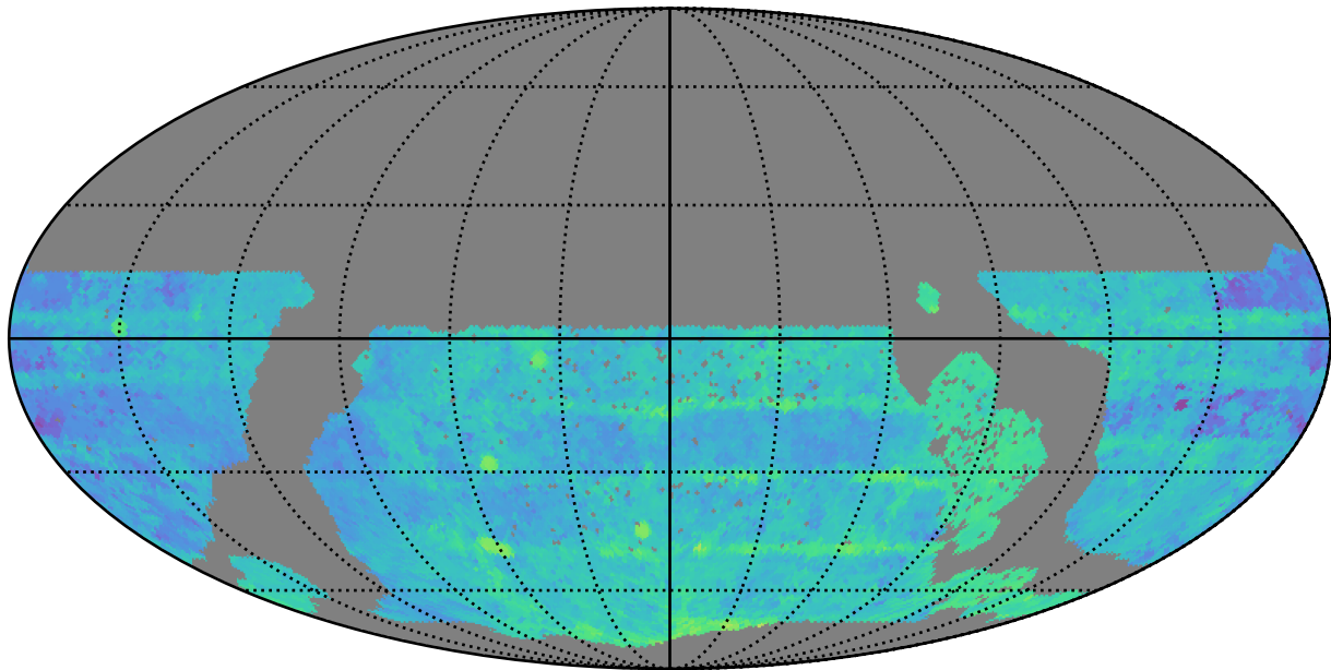
ddf_loaded_fl8_v3.4_10yrs WFD r band: Median Season Length
