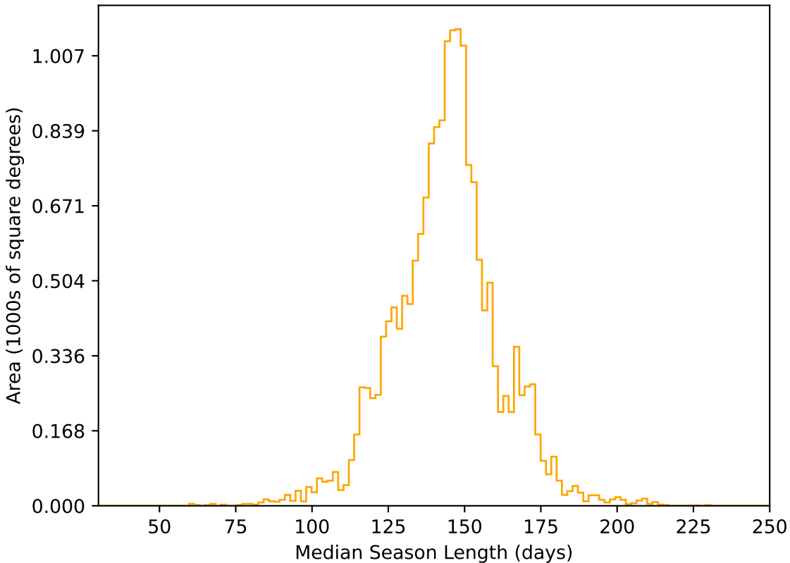
ddf_loaded_fl8_v3.4_10yrs WFD r band: Median Season Length
