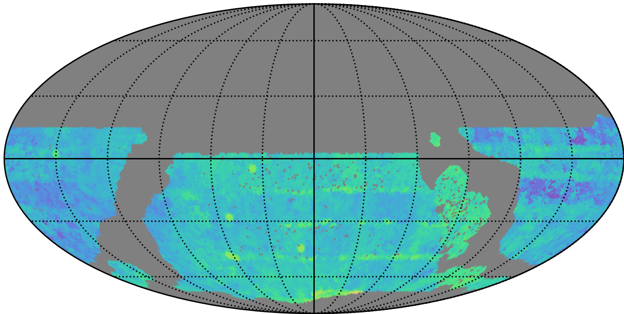
ddf_loaded_fl8_v3.4_10yrs WFD i band: Median Season Length
