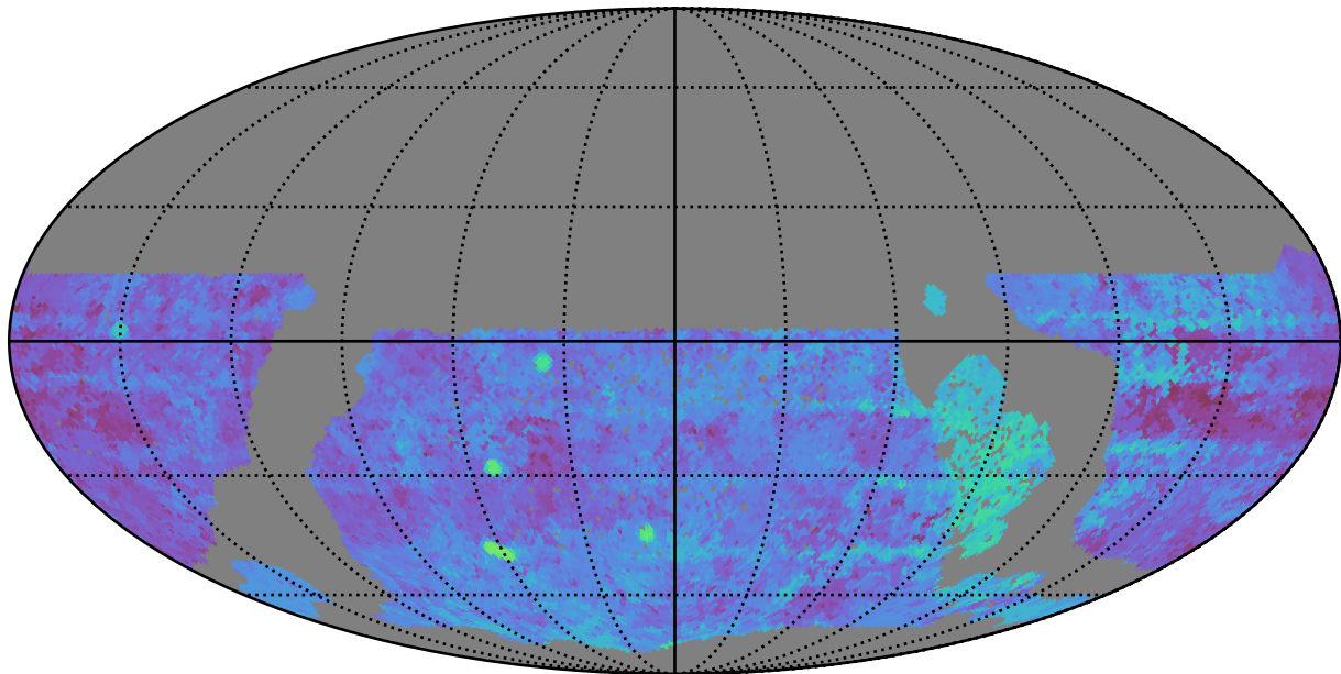
ddf_loaded_fl8_v3.4_10yrs WFD g band: Median Season Length
