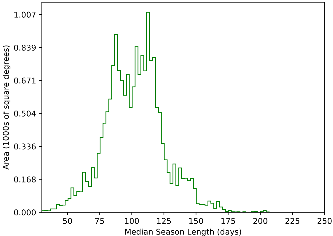
ddf_loaded_fl8_v3.4_10yrs WFD g band: Median Season Length
