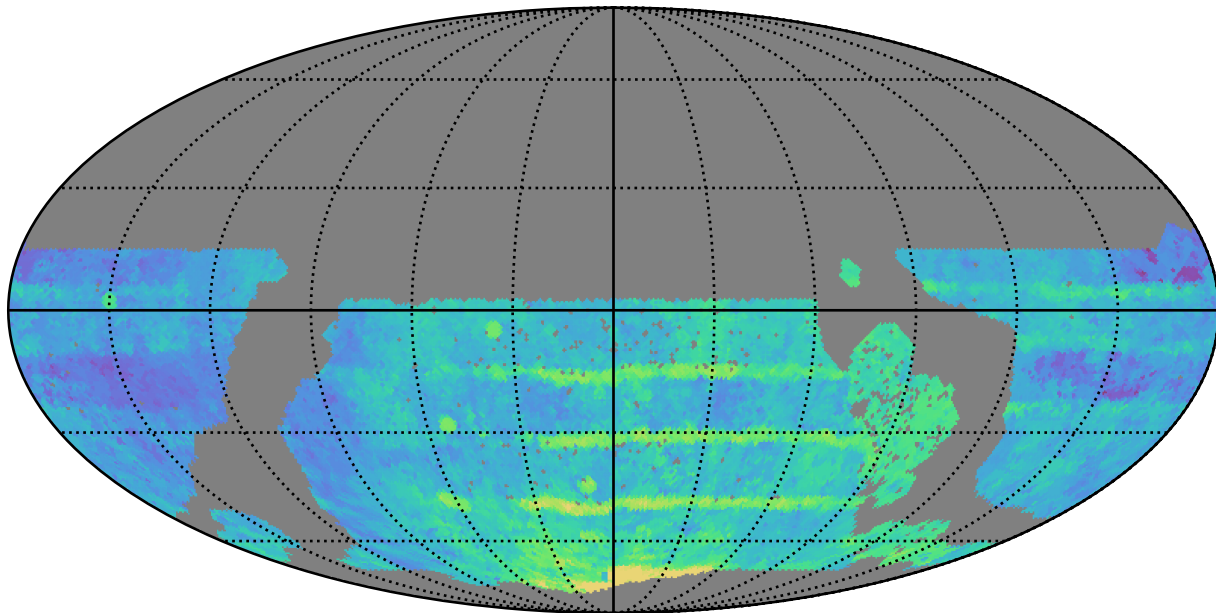
ddf_loaded_fl8_v3.4_10yrs WFD all bands: Median Season Length
