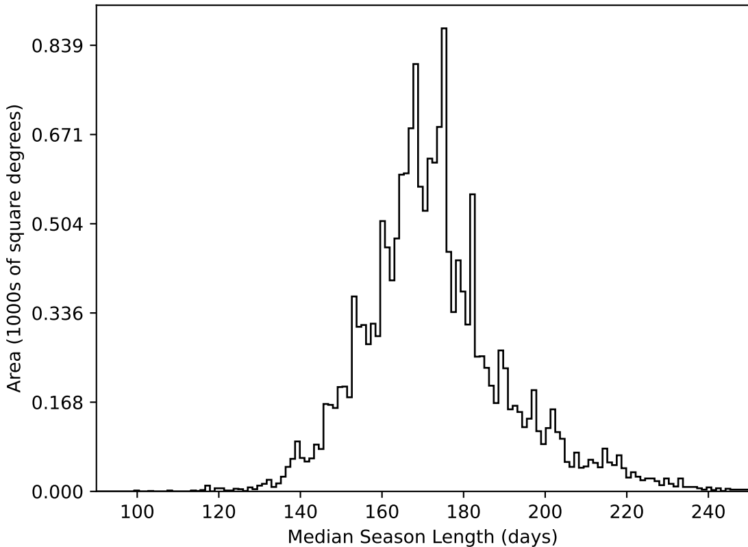
ddf_loaded_fl8_v3.4_10yrs WFD all bands: Median Season Length
