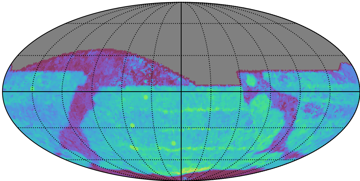
ddf_loaded_fl8_v3.4_10yrs All sky z band: Median Season Length
