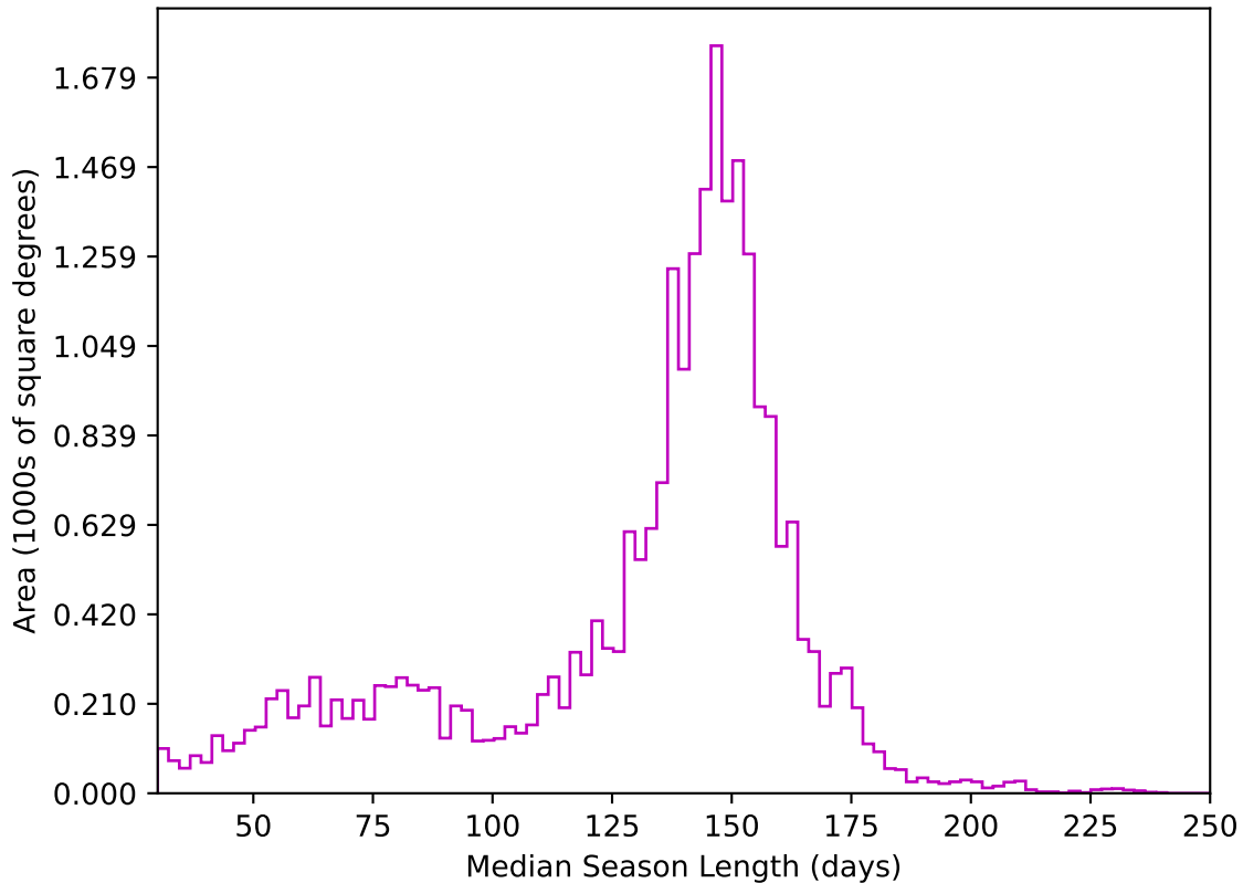
ddf_loaded_fl8_v3.4_10yrs All sky z band: Median Season Length
