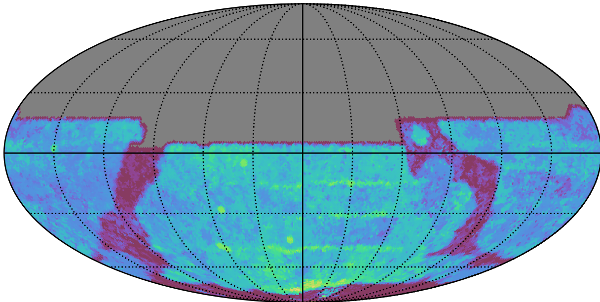
ddf_loaded_fl8_v3.4_10yrs All sky y band: Median Season Length
