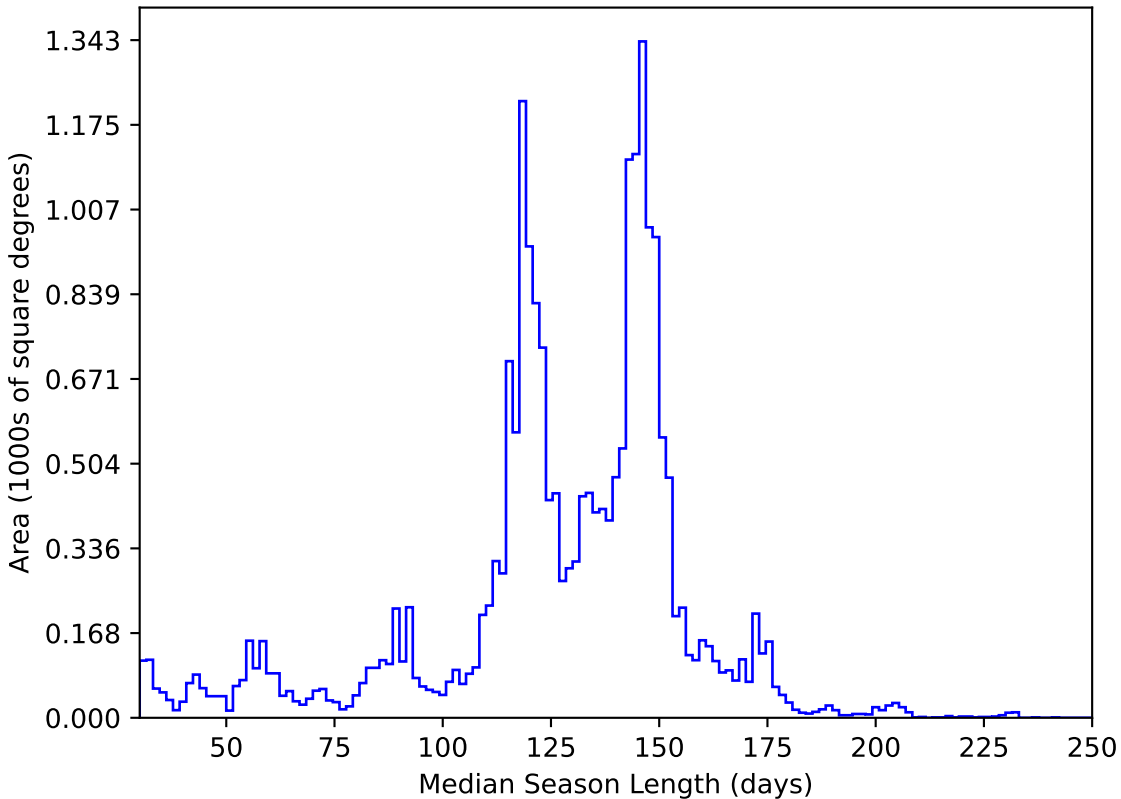
ddf_loaded_fl8_v3.4_10yrs All sky y band: Median Season Length
