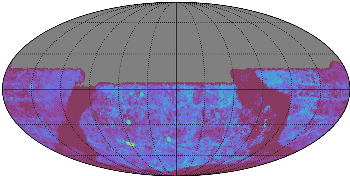
ddf_loaded_fl8_v3.4_10yrs All sky u band: Median Season Length
