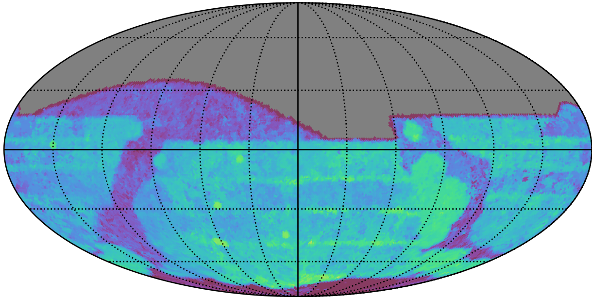
ddf_loaded_fl8_v3.4_10yrs All sky r band: Median Season Length
