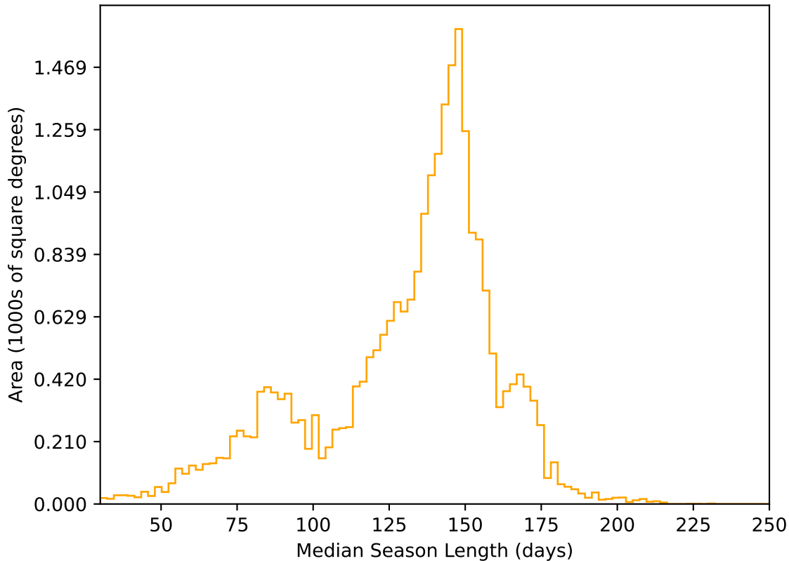
ddf_loaded_fl8_v3.4_10yrs All sky r band: Median Season Length
