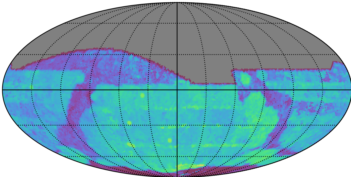
ddf_loaded_fl8_v3.4_10yrs All sky i band: Median Season Length
