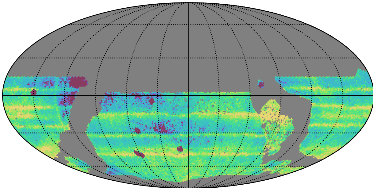
ddf_loaded_fl8_v3.4_10yrs WFD: Median Intra-Night Gap
