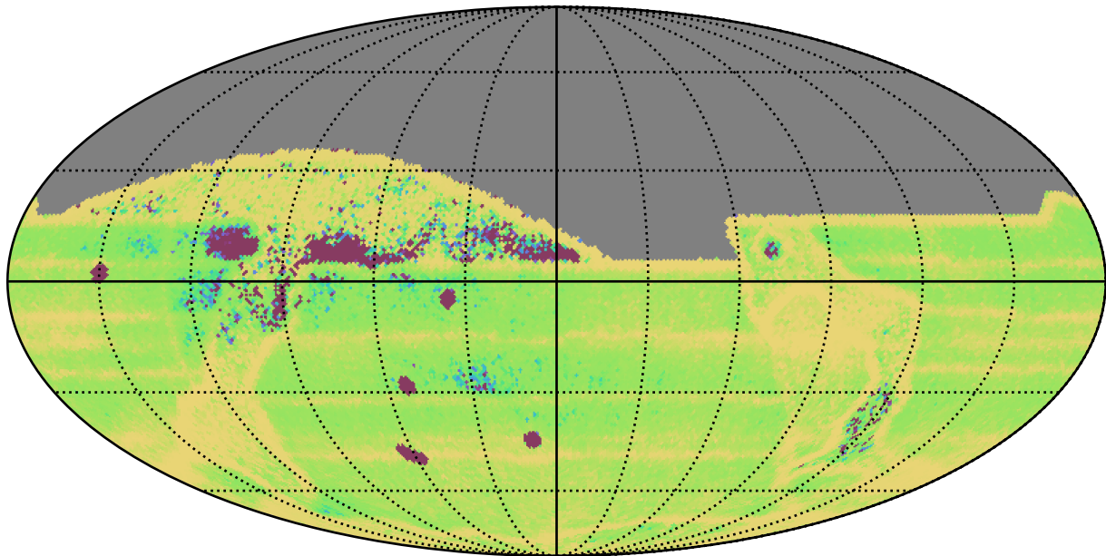
ddf_loaded_fl8_v3.4_10yrs All sky: Median Intra-Night Gap
