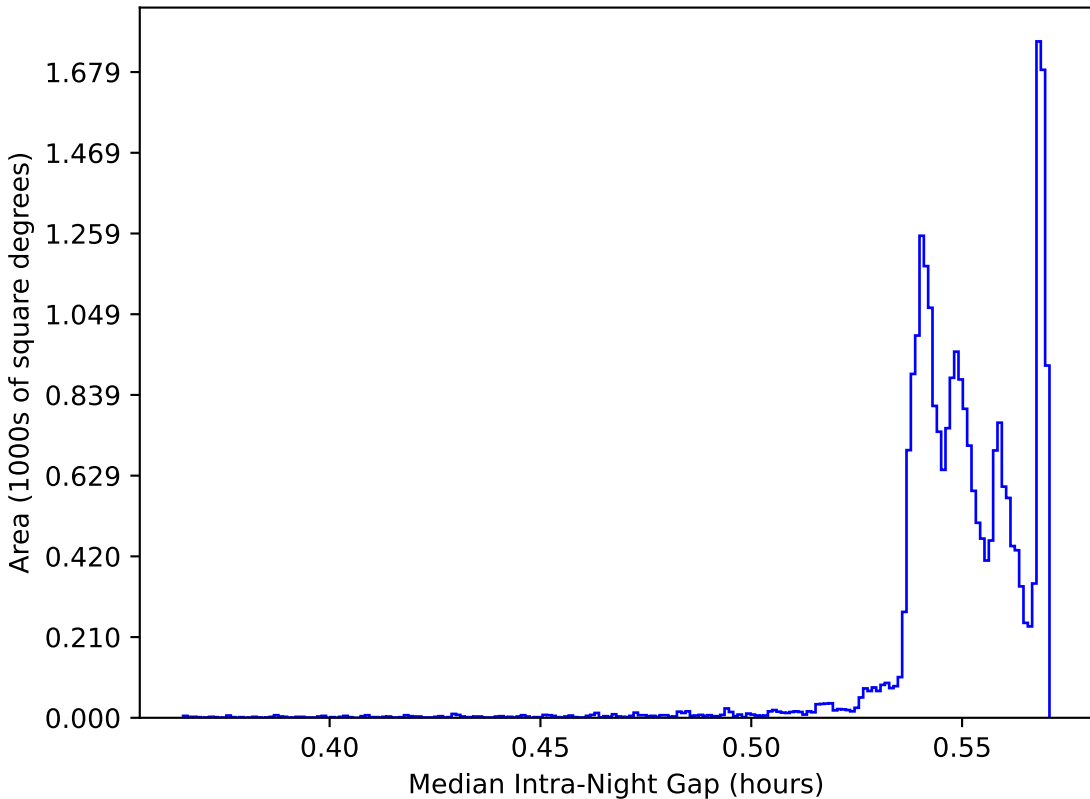
ddf_loaded_fl8_v3.4_10yrs All sky: Median Intra-Night Gap
