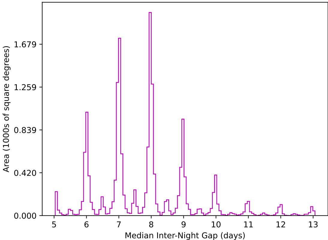
ddf_loaded_fl8_v3.4_10yrs WFD z band: Median Inter-Night Gap
