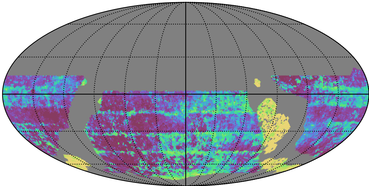
ddf_loaded_fl8_v3.4_10yrs WFD y band: Median Inter-Night Gap
