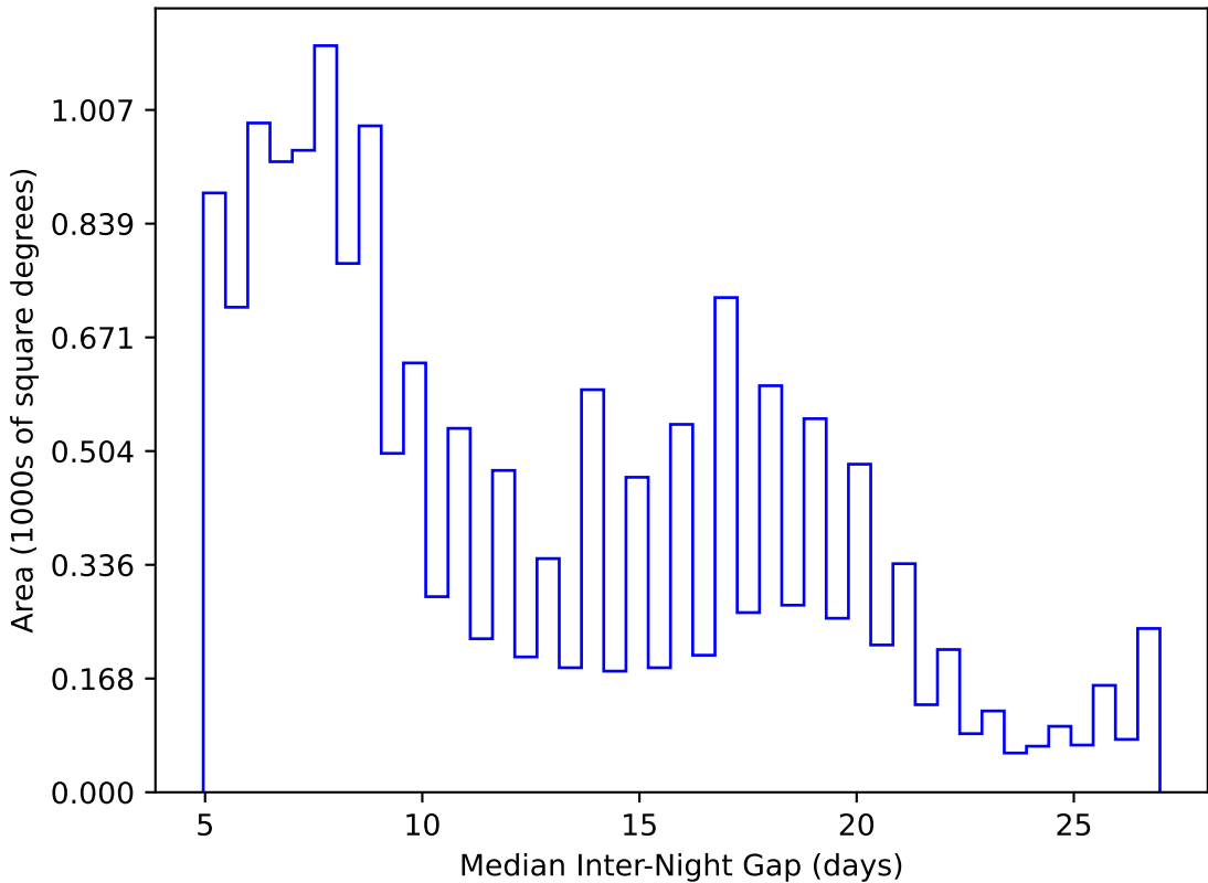
ddf_loaded_fl8_v3.4_10yrs WFD y band: Median Inter-Night Gap
