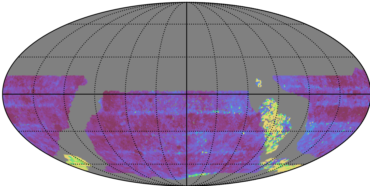
ddf_loaded_fl8_v3.4_10yrs WFD u band: Median Inter-Night Gap
