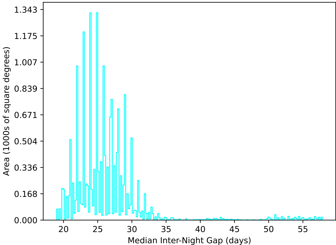
ddf_loaded_fl8_v3.4_10yrs WFD u band: Median Inter-Night Gap
