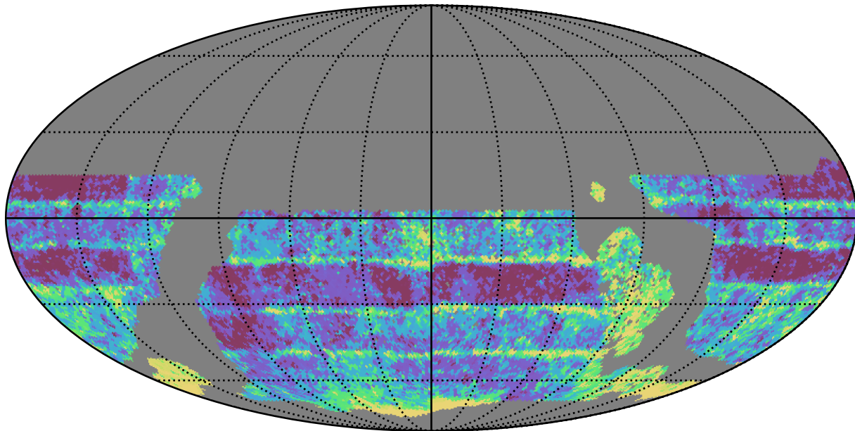
ddf_loaded_fl8_v3.4_10yrs WFD r band: Median Inter-Night Gap
