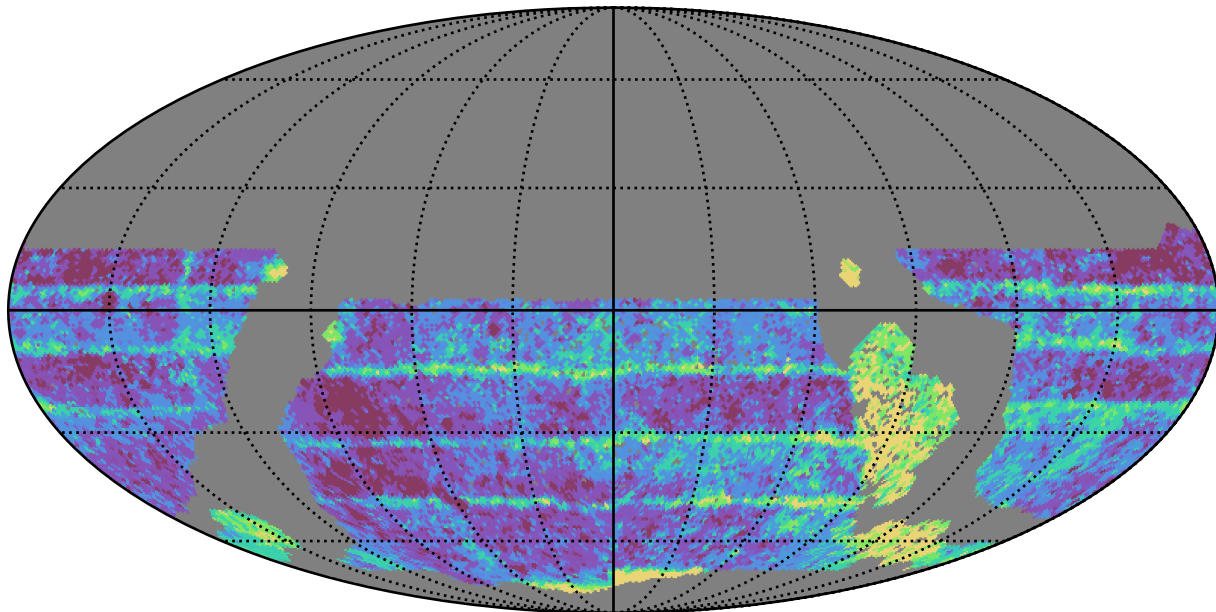
ddf_loaded_fl8_v3.4_10yrs WFD i band: Median Inter-Night Gap
