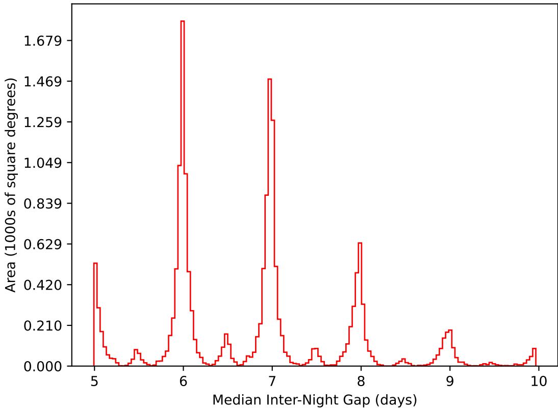
ddf_loaded_fl8_v3.4_10yrs WFD i band: Median Inter-Night Gap
