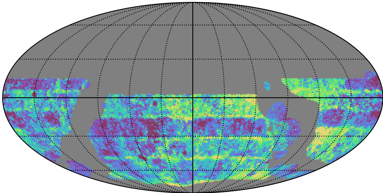
ddf_loaded_fl8_v3.4_10yrs WFD g band: Median Inter-Night Gap
