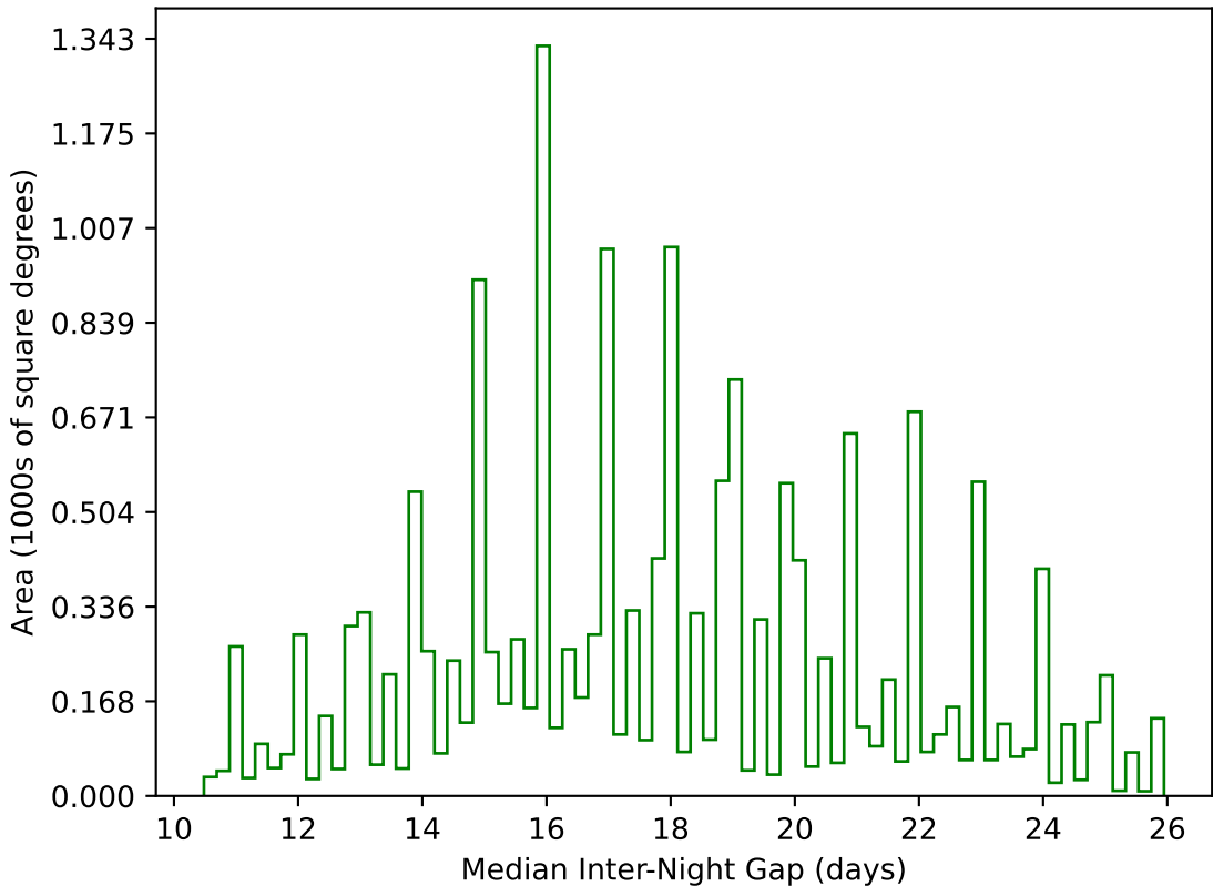
ddf_loaded_fl8_v3.4_10yrs WFD g band: Median Inter-Night Gap
