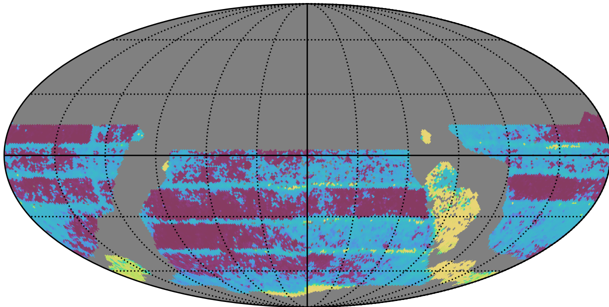
ddf_loaded_fl8_v3.4_10yrs WFD all bands: Median Inter-Night Gap
