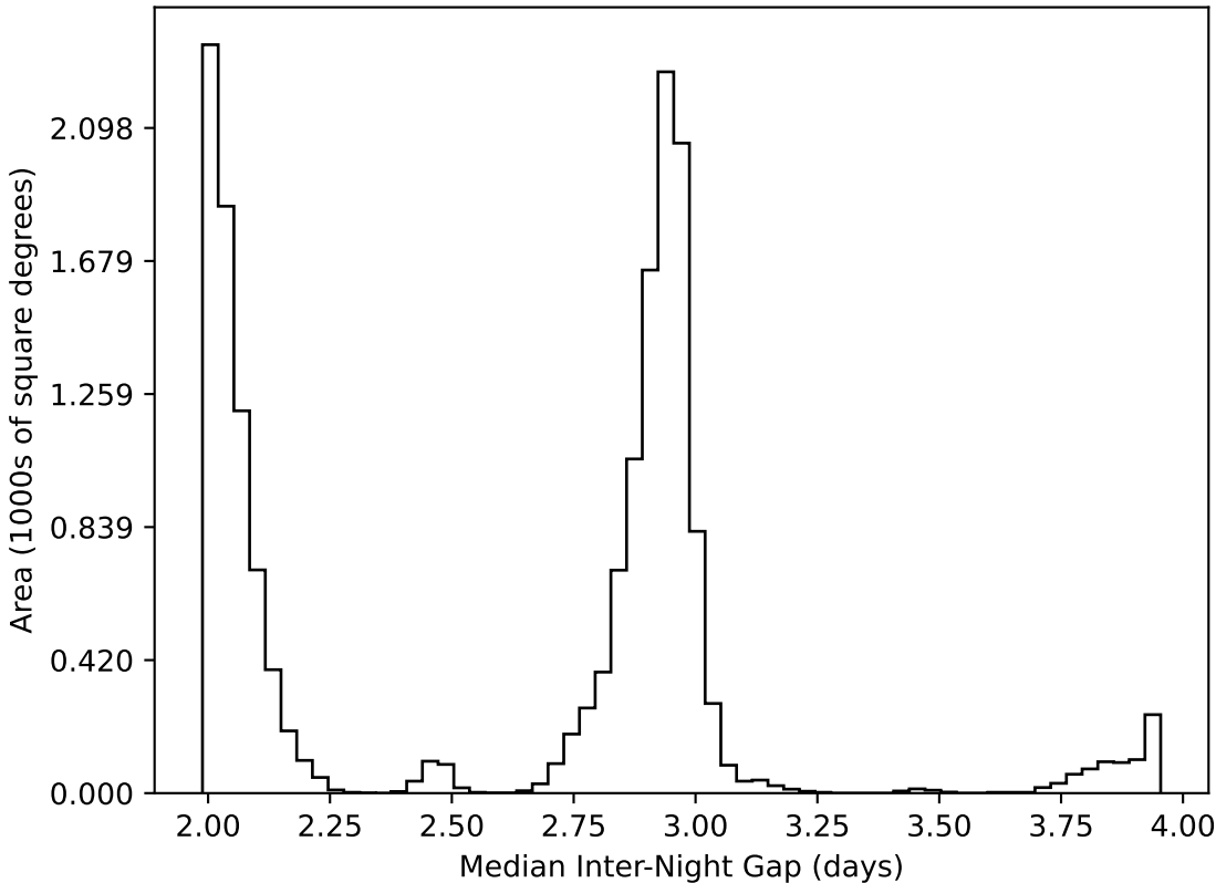
ddf_loaded_fl8_v3.4_10yrs WFD all bands: Median Inter-Night Gap
