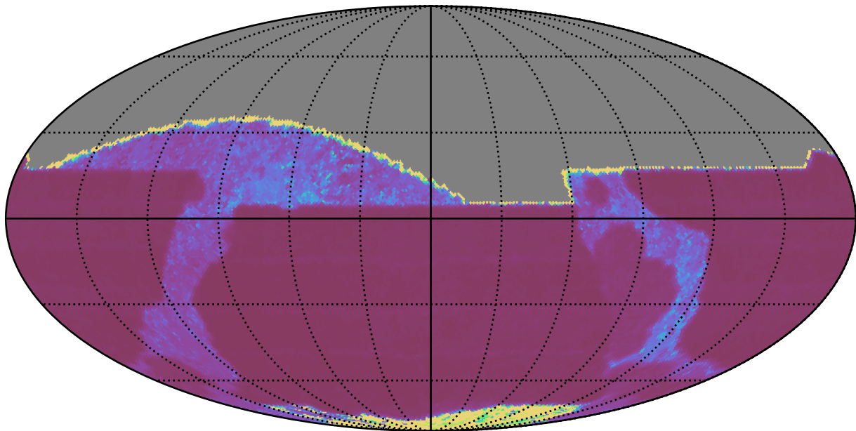
ddf_loaded_fl8_v3.4_10yrs All sky z band: Median Inter-Night Gap
