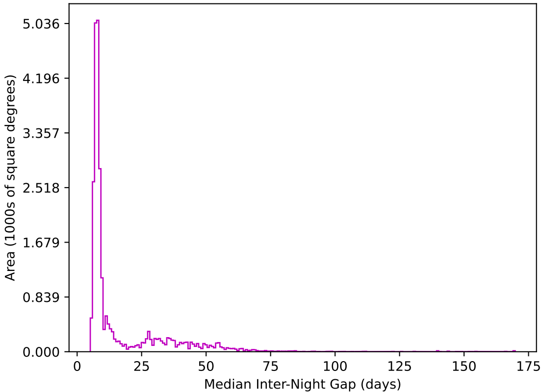
ddf_loaded_fl8_v3.4_10yrs All sky z band: Median Inter-Night Gap
