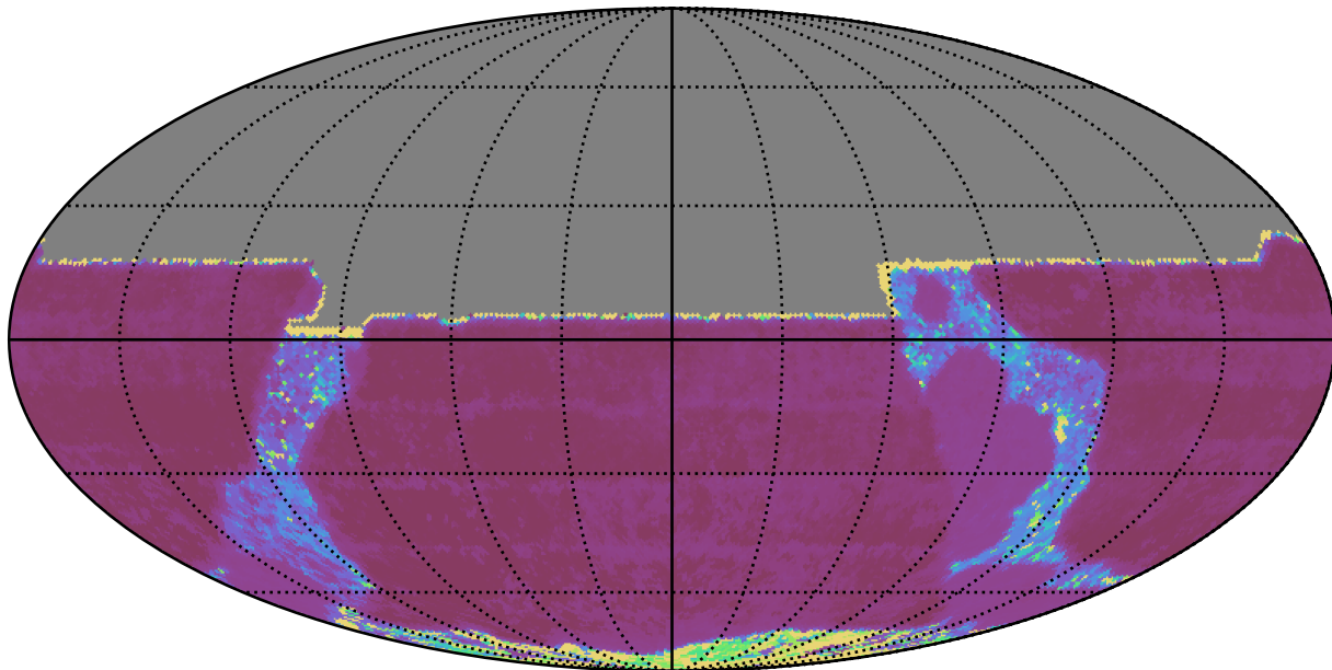
ddf_loaded_fl8_v3.4_10yrs All sky y band: Median Inter-Night Gap
