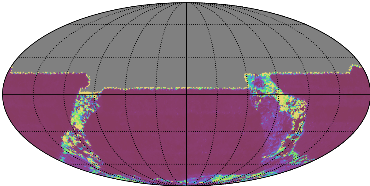
ddf_loaded_fl8_v3.4_10yrs All sky u band: Median Inter-Night Gap
