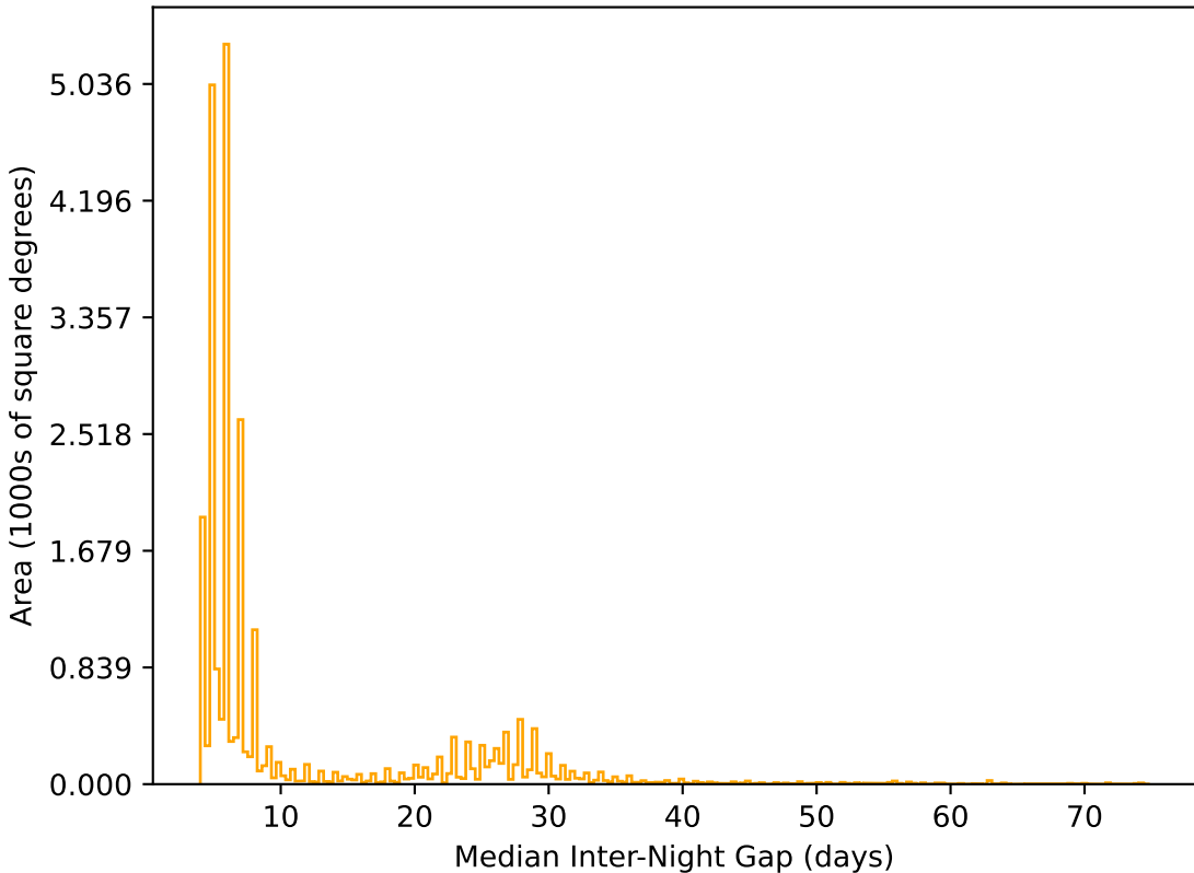
ddf_loaded_fl8_v3.4_10yrs All sky r band: Median Inter-Night Gap
