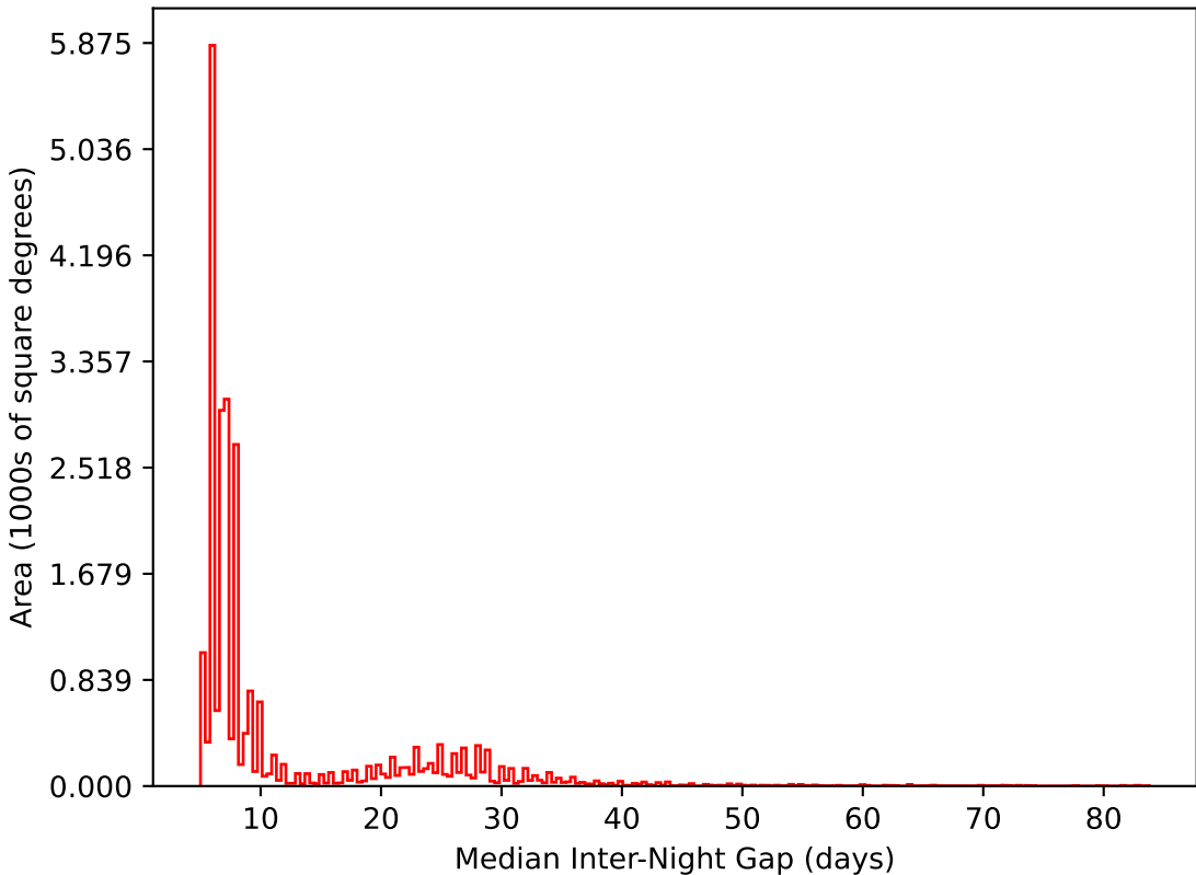
ddf_loaded_fl8_v3.4_10yrs All sky i band: Median Inter-Night Gap
