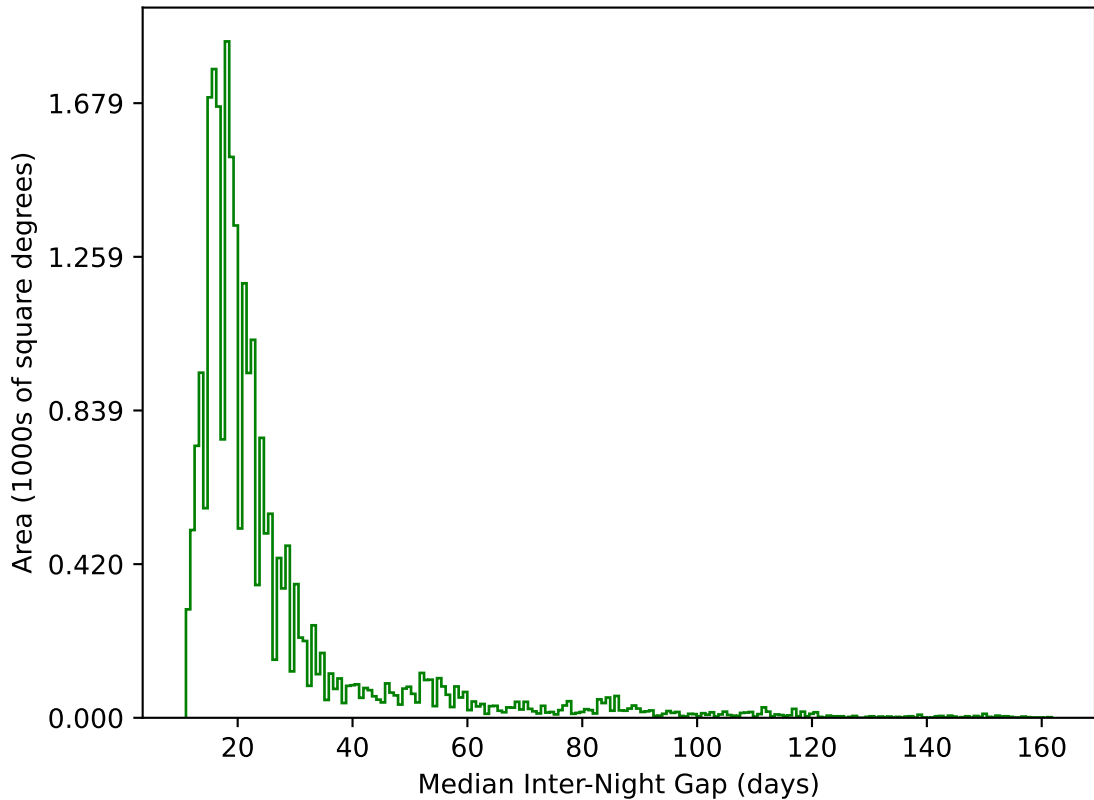
ddf_loaded_fl8_v3.4_10yrs All sky g band: Median Inter-Night Gap
