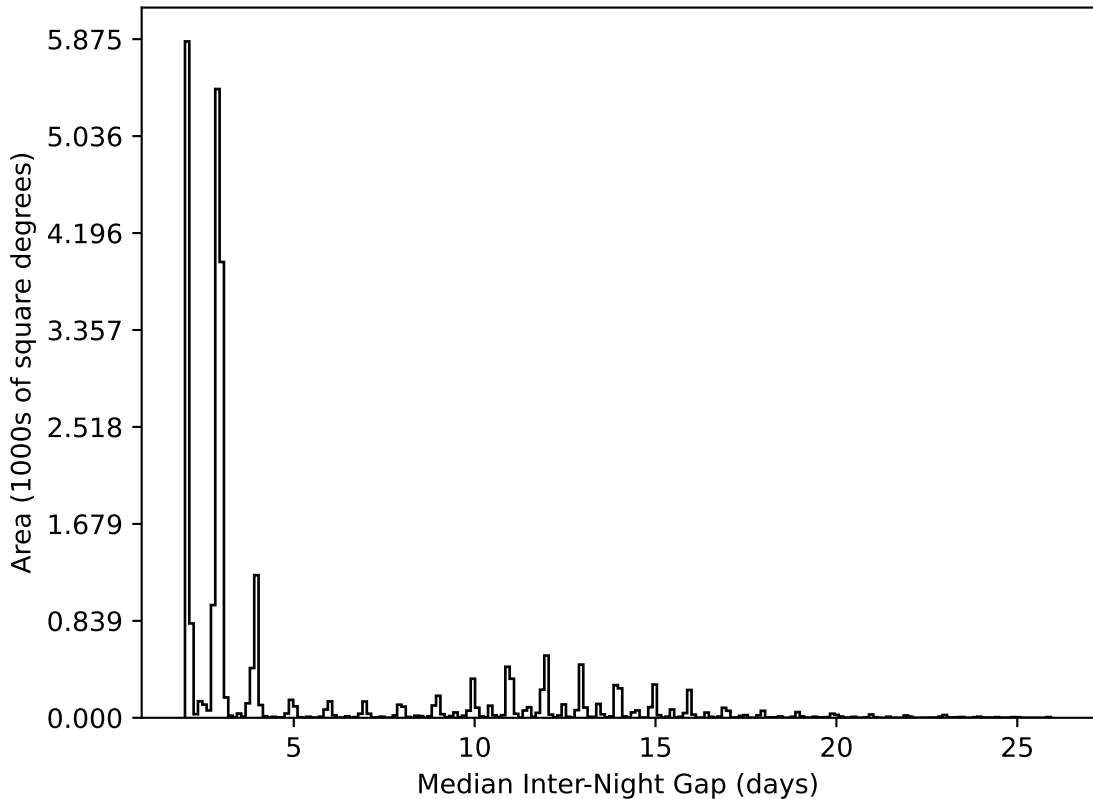
ddf_loaded_fl8_v3.4_10yrs All sky all bands: Median Inter-Night Gap
