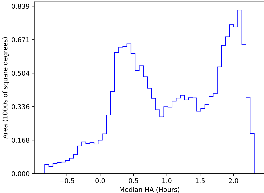
ddf_loaded_fl8_v3.4_10yrs WFD z band: Median HA
