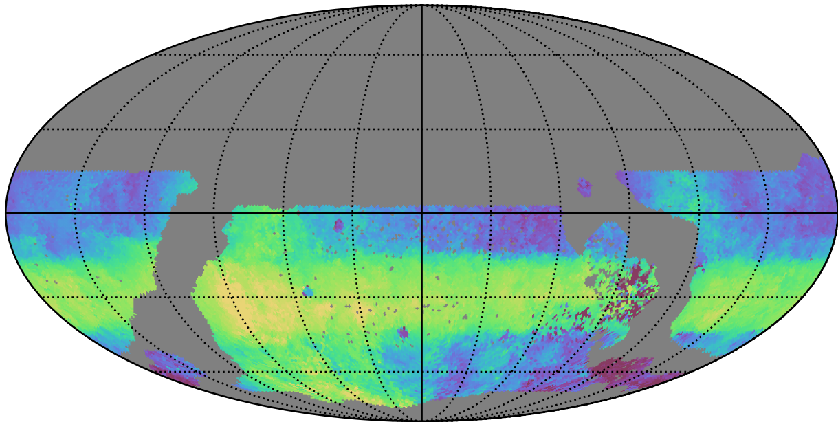
ddf_loaded_fl8_v3.4_10yrs WFD u band: Median HA
