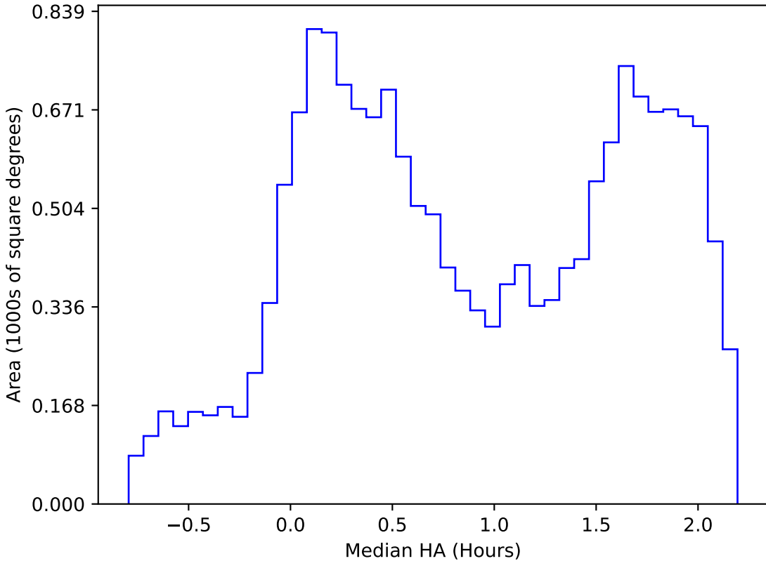
ddf_loaded_fl8_v3.4_10yrs WFD r band: Median HA
