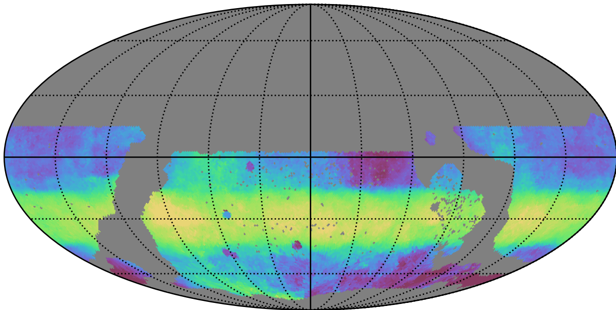
ddf_loaded_fl8_v3.4_10yrs WFD i band: Median HA
